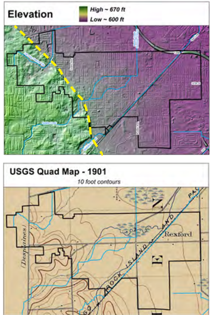
FIGURE 4 AND 5: ELEVATION; USGS QUAD MAP Map courtesy of the US Army Corps of Engineers
