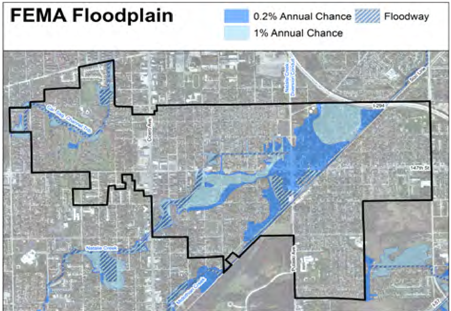
FIGURE 14: FEMA FLOODPLAIN Map courtesy of the US Army Corps of Engineers
